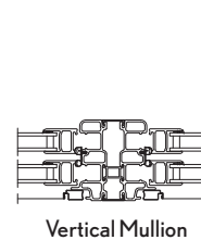
Vertical Mullion
